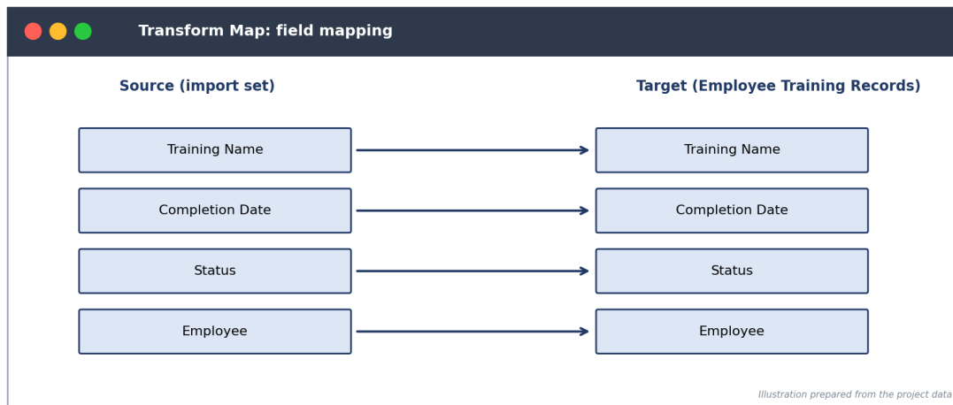
Figure 2: Data preprocessing - Transform Map field mapping (illustration)
